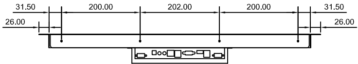
BOTTOM VIEW
